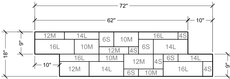
Wall Pattern 1 Front Elevation View
