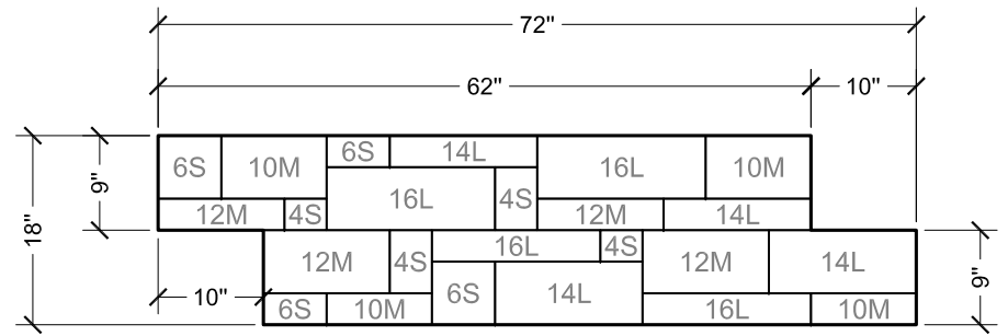
Wall Pattern 2 Front Elevation View
