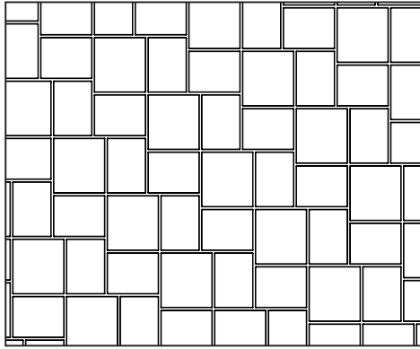
2:1 Herringbone Pattern 6x6 (25%), 6x9 (75%)
