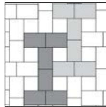
"I" Pattern 25% 6x6 Square 75% 6x9 Rectangle
