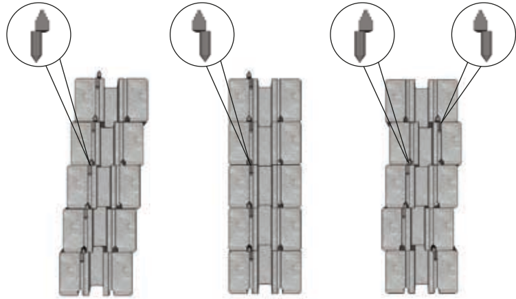
Batter (Setback) 4.5° Flag in Back Position
