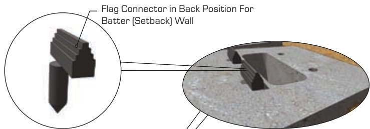
Shadow (Multi-Setback) Flag in Forward and Backward Position
