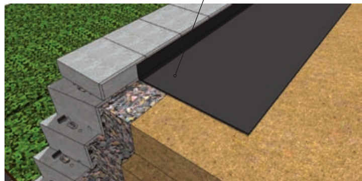
Soil Separating Filter Fabric
